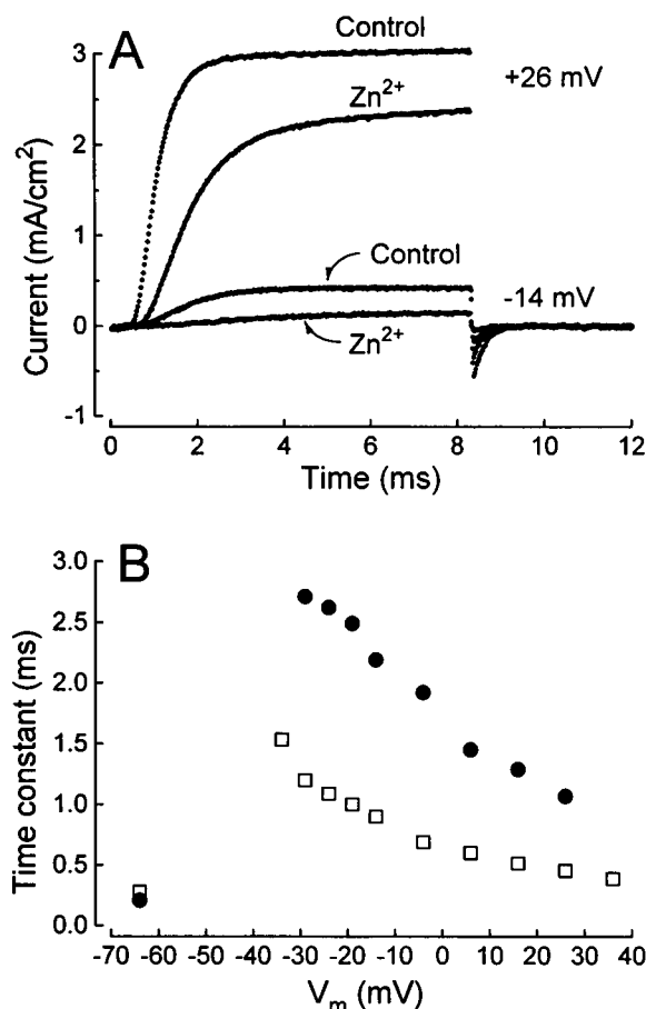
FIGURE 7 External \text{Zn}^{2+} and K channel ionic currents. (A) Raw currents recorded (20°C) at depolarizations to -14 and +26 mV before and during exposure to 10 mM external \text{Zn}^{2+} in Tris- \text{NO}_3 ASW without Cs. (B) Activation and deactivation (at -64 mV) time constants in the absence (○) and in the presence of external \text{Zn}^{2+} (●).
