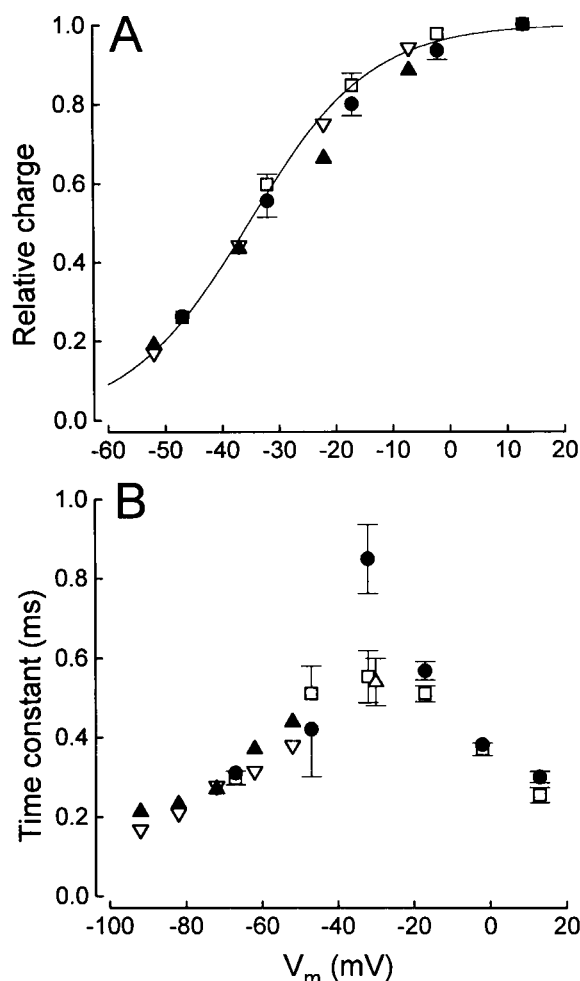
FIGURE 5 Internal \text{Zn}^{2+} and charge movement and gating current kinetics. Mean ( \square , \bullet ) and SEM values from four axons; SEM limits not shown if smaller than symbol. ( \nabla , \blacktriangle ) Average data from two additional axons. (A) Voltage dependence of relative gating charge movement. Line: fit of Eq. 1 to the data in the absence of \text{Zn}^{2+} . Fitted values: q = 2.3 e; V_{1/2} = -35 mV. (B) Gating current ON (for potentials more positive than -60 mV) and OFF-time constants. The ON-time constant at -32 mV (D) recorded after \text{Zn}^{2+} washout has been displaced slightly along the voltage axis for clarity.
