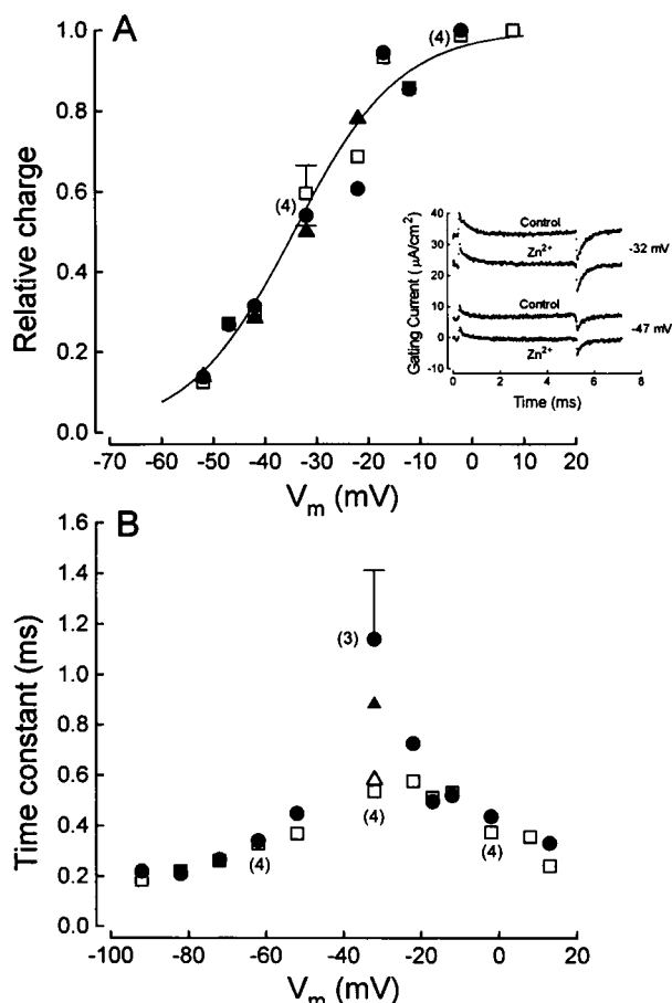
FIGURE 8 External \text{Zn}^{2+} and K channel-gating currents. (A) Voltage dependence of relative charge moved in the absence (□) and presence of external \text{Zn}^{2+} (●). Mean values from four axons as indicated; the remaining data are average values from two additional axons. SEM limits shown where larger than the symbols. Charge movement at -52 , -42 , -32 , and -22 mV were obtained in the presence of \text{Zn}^{2+} from an axon not treated with 4-AP. These values were normalized (▲) by the extrapolated maximum value obtained from a fit of a Boltzmann function. (inset) Raw gating current records in the absence ("Control") and presence of internal \text{Zn}^{2+} recorded at -47 and -32 mV. (B) Gating current ON (for potentials more positive than -50 mV) and OFF-time constants in the absence (□) and presence (●) of external \text{Zn}^{2+} . Where indicated, values are the average of data from four axons. SEM limits shown where larger than the symbols. Data at -32 mV in the absence (△) and presence (▲) of \text{Zn}^{2+} from an axon not treated with 4-AP are included.
