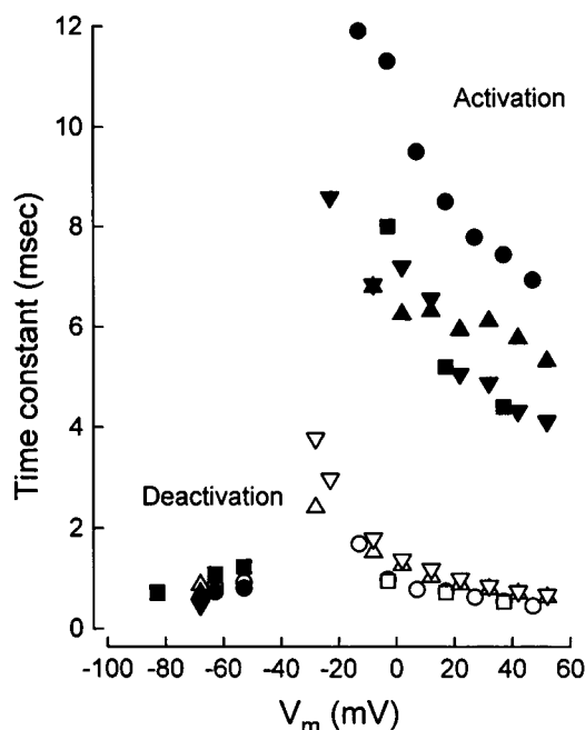
FIGURE 2 Internal \text{Zn}^{2+} and squid axon ionic current time constants. Activation and deactivation (for V_m more negative than -40 mV) obtained from exponential fits to data. Open symbols in the absence and filled symbols in the presence of internal \text{Zn}^{2+} . Data from four axons identified by different symbols. The concentration of free \text{Zn}^{2+} concentration was near 200–300 nM (see Materials and Methods).
